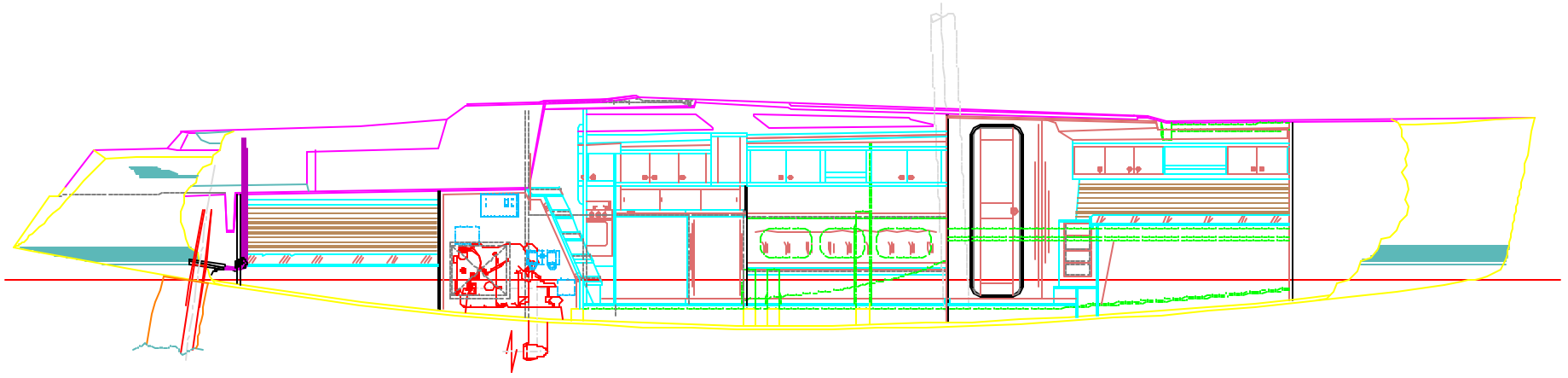
BALTIC 50' interior layout version II
